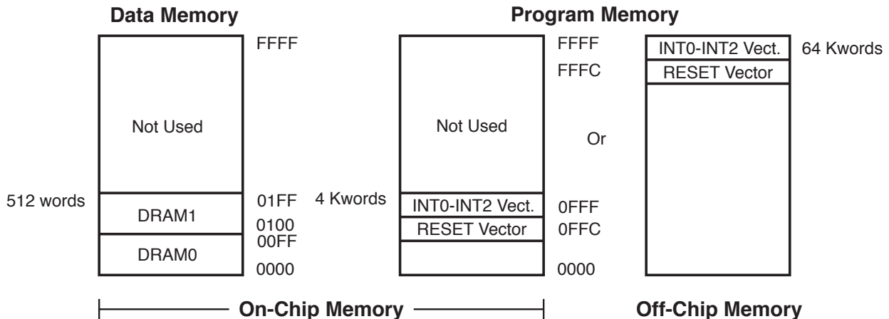
Figure 15. Memory Map
